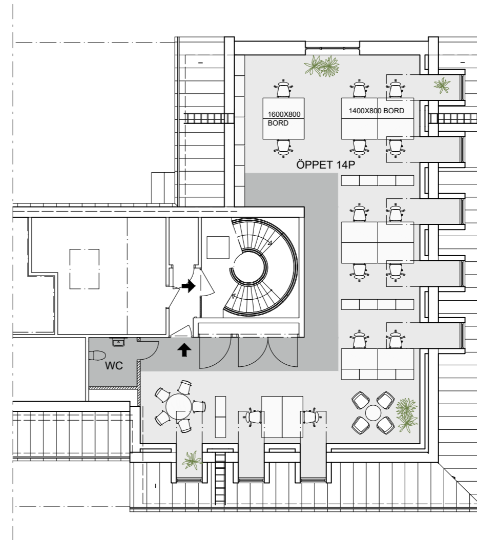
PLAN 9 ca 120 m 2
